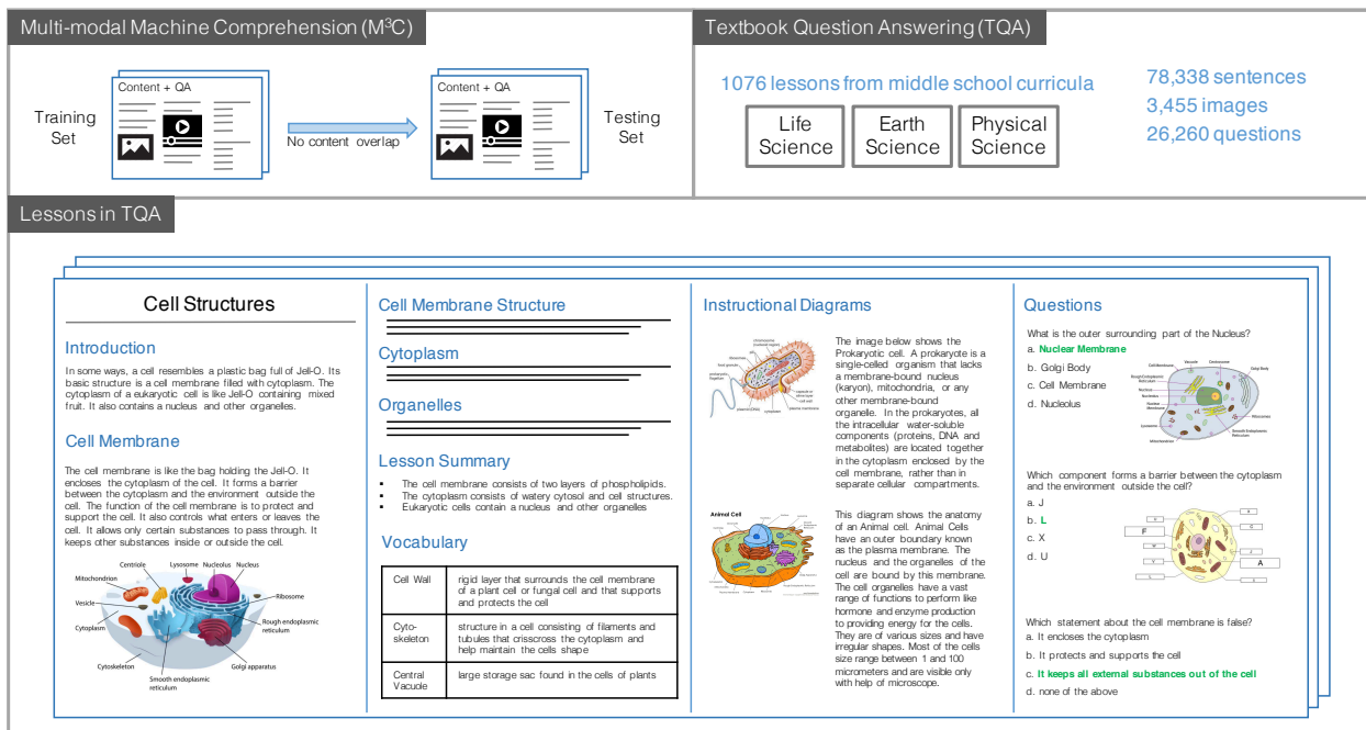
Figure 1. An overview of the Multi-modal Machine Comprehension (M³C) paradigm, statistics of the proposed Textbook Question Answering (TQA) dataset and an illustration of a lesson in it. TQA can be downloaded at http://textbookqa.org .
