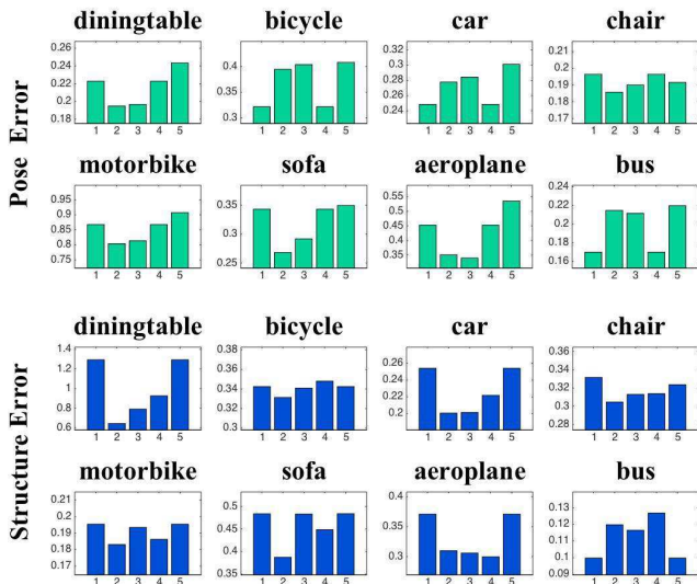
Figure 5. Evaluating our method using PASCAL3D+ natural images in terms of pose error (top), and structure error (bottom). The x-axis shows the results of (1) landmark registration, (2) silhouette fitting with all components, (3) silhouette fitting without \ell_2 regularization, (4) silhouette fitting without camera refinement, and (5) silhouette fitting without dense model combination.
