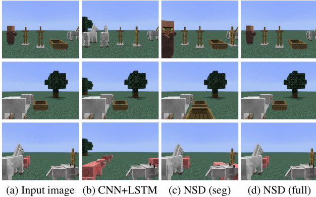
(a) Input image (b) CNN+LSTM (c) NSD (seg) (d) NSD (full) Figure 9: Results on the Minecraft dataset. From left to right: (a) input images, and results of (b) the CNN+LSTM model, (c) our de-rendering framework with segment proposals, and (d) our full model with REINFORCE and analysis-by-synthesis. See Section 4.1 for details of these methods and Section 4.3 for analyses.
