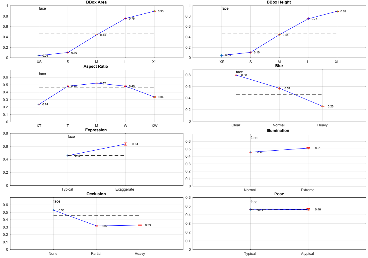
Figure 3: Sensitivity and impact of object characteristics. We show normalized AP[1] for each characteristics. Please refer to [1] for definition of “BBox Area”, “BBox Height”, and “Aspect Ratio” and also refer to [5] for the definition of per-face attributes “Blur”, “Expression”, “Illumination”, “Occlusion”, and “Pose”. Our detector performs under average in the case of extremely small scale, extremely skewed aspect ratio, heavy blur, and heavy occlusion. Surprisingly, exaggerated expression and extreme illumination correlate with better performance. Pose variation does not have noticeable affect.
