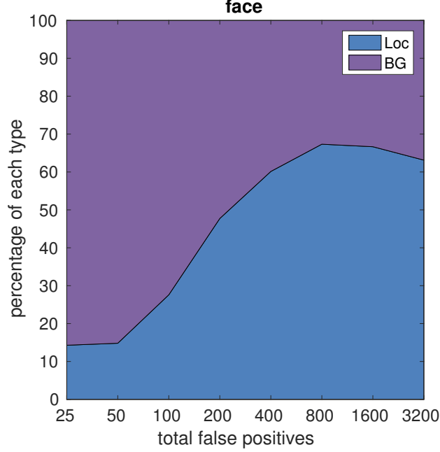
Figure 1: Distribution of error modes of false positives. Background confusion seems the dominating error mode among top-scoring detection, however, we found 15 out of 20 top-scoring false positives, as shown in Fig. 4, are in fact due to missed annotation.
