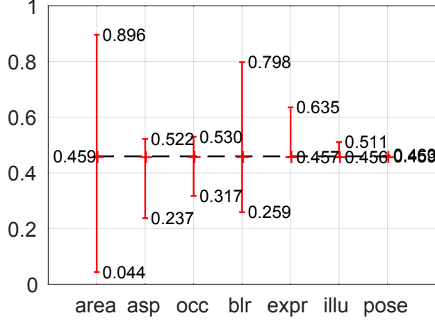
Figure 2: Summary of sensitivity plot. We plot the maximum and minimum of AP_N shown in Figure 3. Our detector is mostly affected by object scale (from 0.044 to 0.896) and blur (from 0.259 to 0.798).
