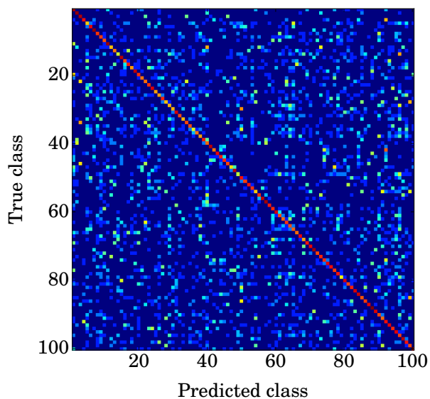
(a) iCaRL
