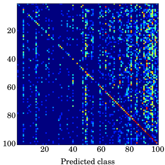
(b) LwF.MC
