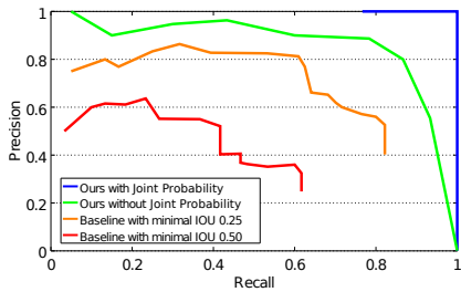
Figure 3. The precision-recall curves for our method with (blue) and without (green) use of the joint probability. The orange and red curves are the baseline method with minimal IOU set to 0.25 and 0.50 respectively.
