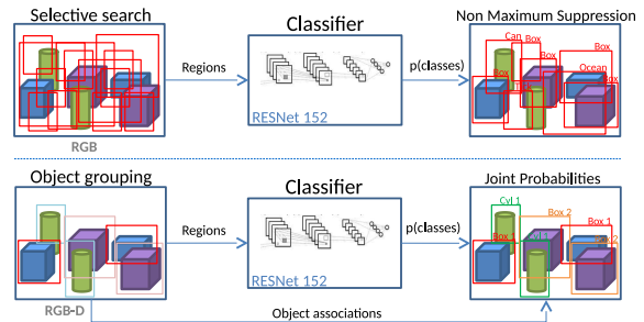
Figure 1. A typical object detection pipeline utilizing a CNN (top), and the proposed pipeline using an alternative object discovery method for region proposal (bottom).
