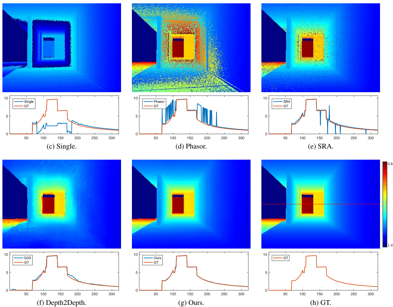
Figure 2: Synthetic results on a long-range scene with relatively high MPI and sensor noise.
