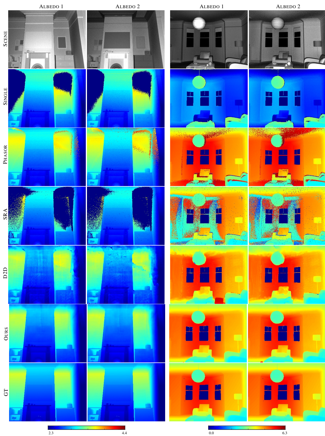
Figure 18: Robustness to albedos on two pairs of synthetic scenes.
