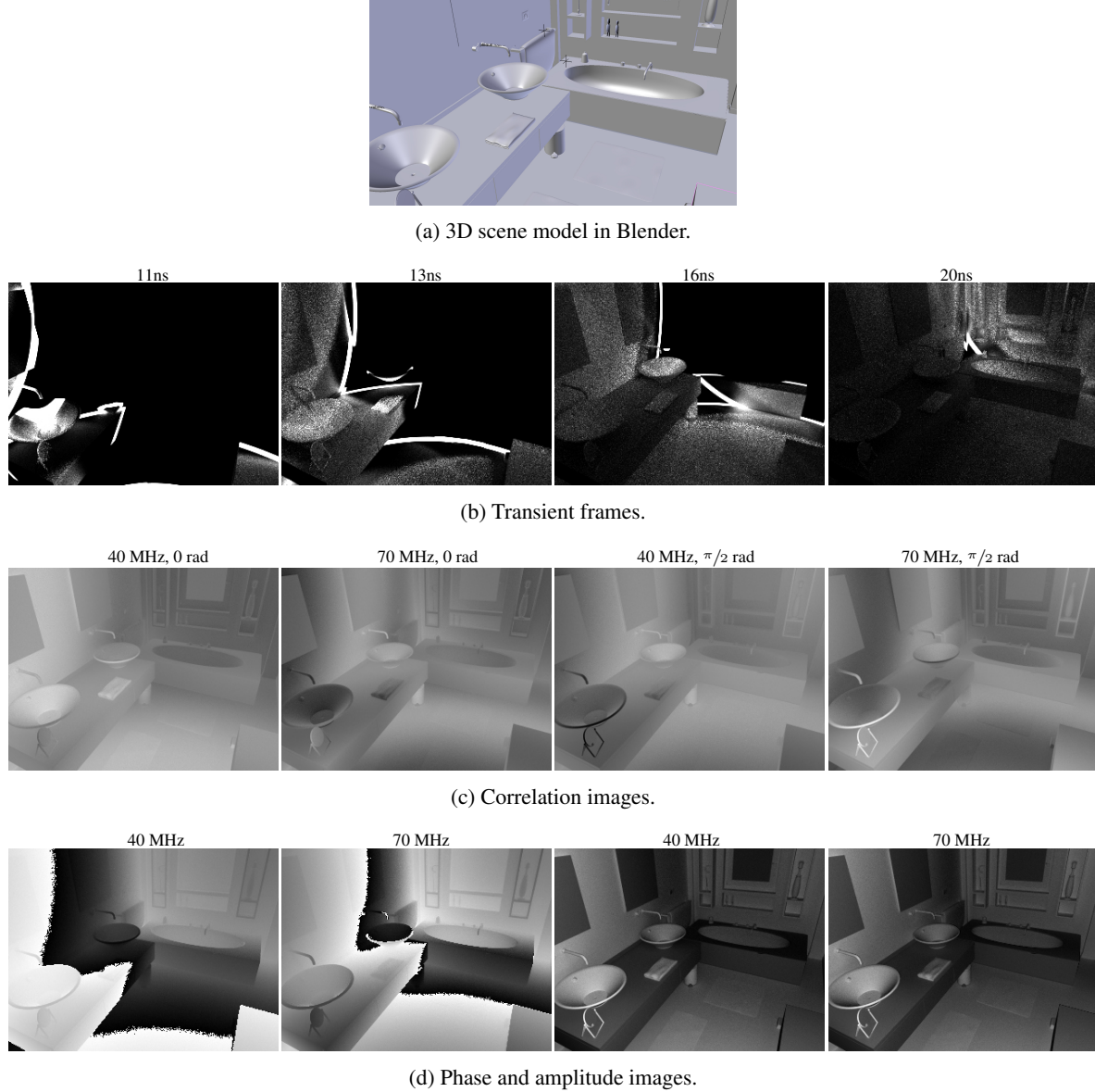
Figure 20: Synthetic data generation steps.
