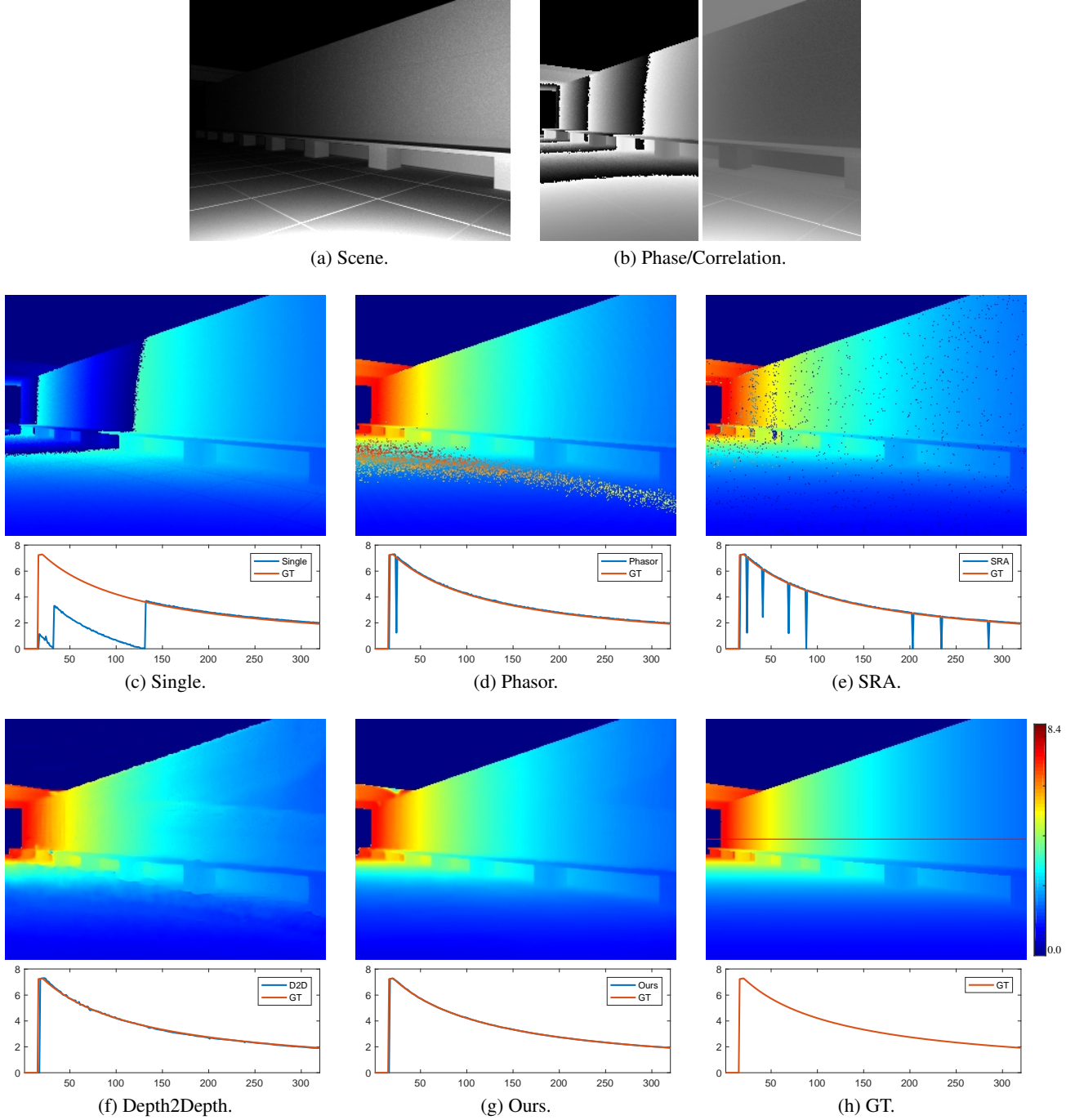
Figure 1: Synthetic results on a long-range scene with relatively low MPI and sensor noise.
