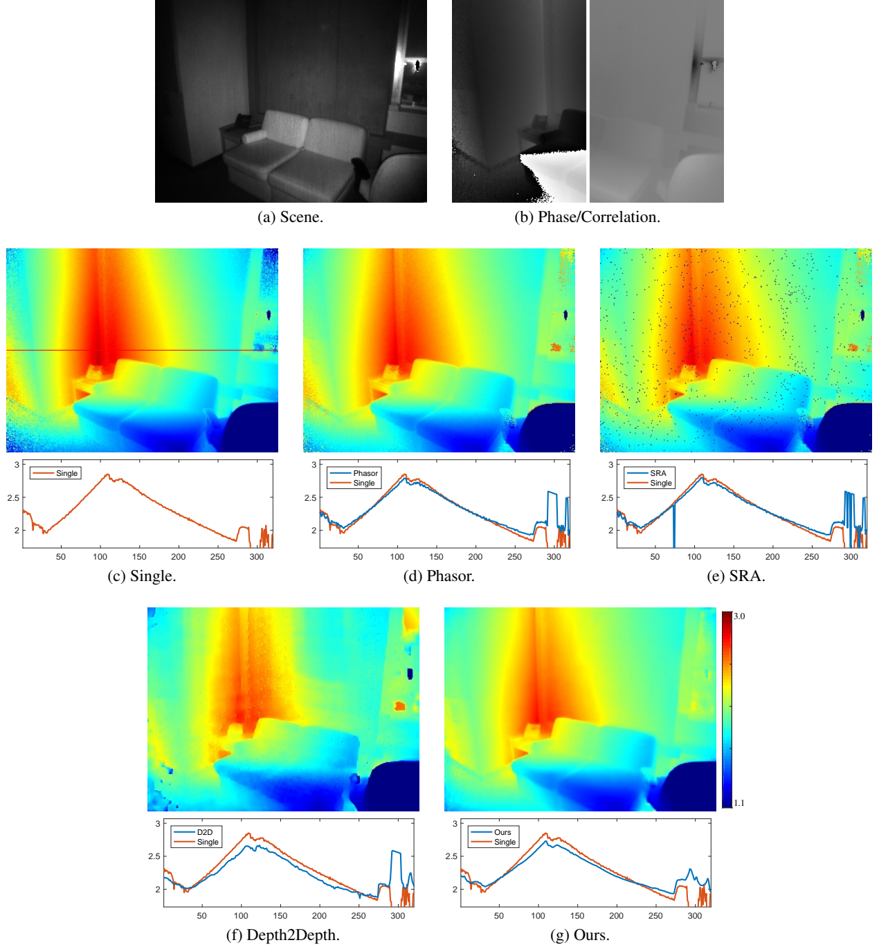
Figure 7: Real results from an office scene consisting of a concrete wall corner, sofa, chair and glass window. Our method generates piecewise smooth depth map while compensating for MPI distortion and glass reflectance.
