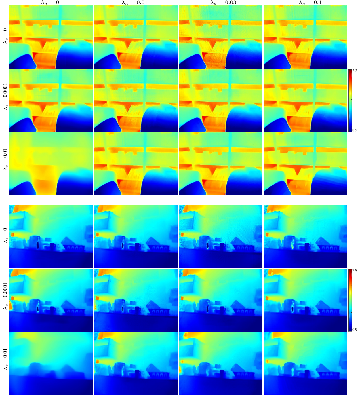
Figure 19: Effect of \lambda_a and \lambda_s variations on two example scenes, BOOKSHELF (top) and KITCHEN (bottom). Results are best seen with a computer.
