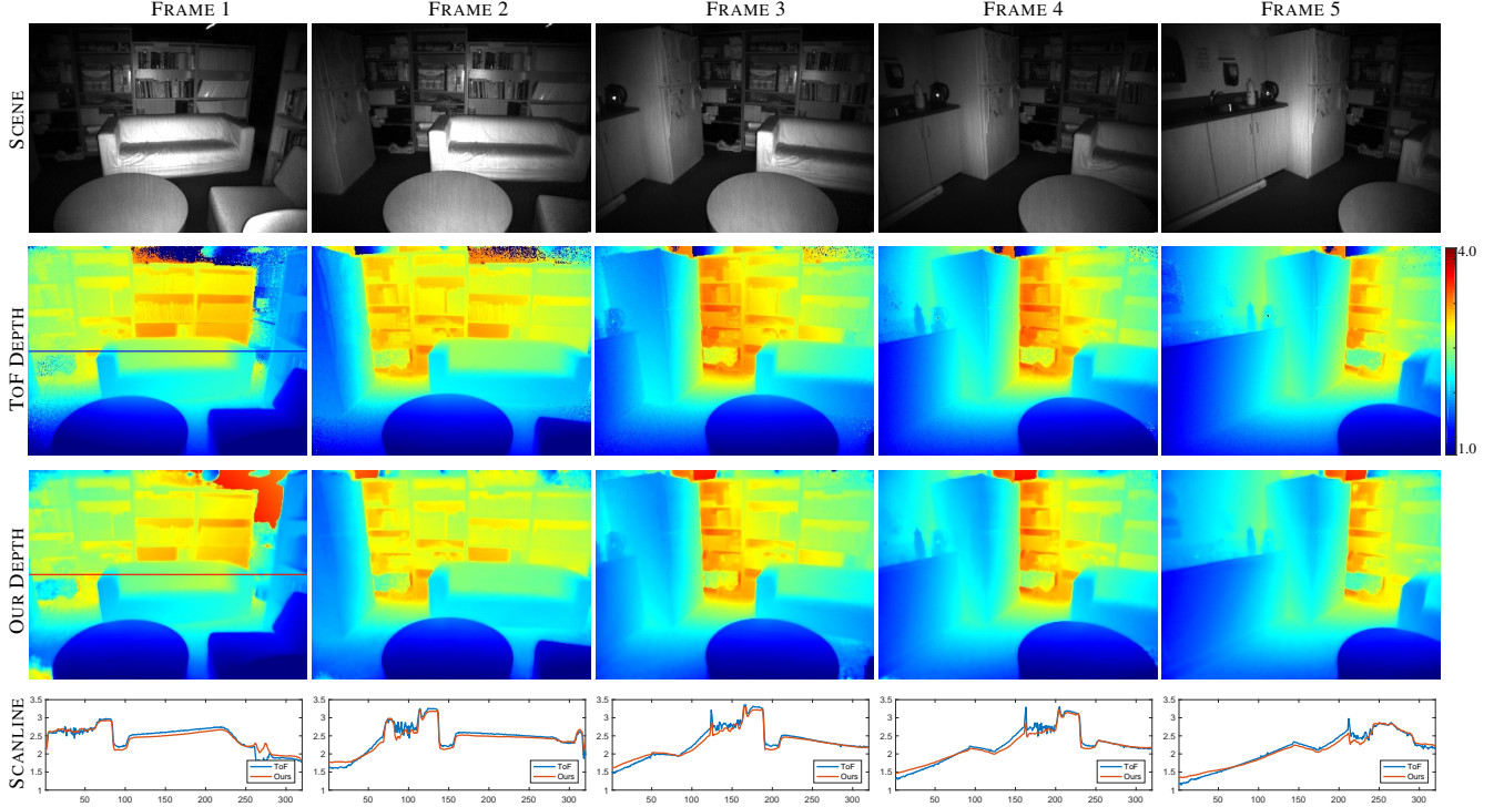
Figure 16: Evaluation of the temporal consistency with experimentally captured raw ToF measurements. We denote TOFDEPTH as the single frequency output measured at \omega_1 = 40 MHz, and OURDEPTH as the results of the proposed framework.
