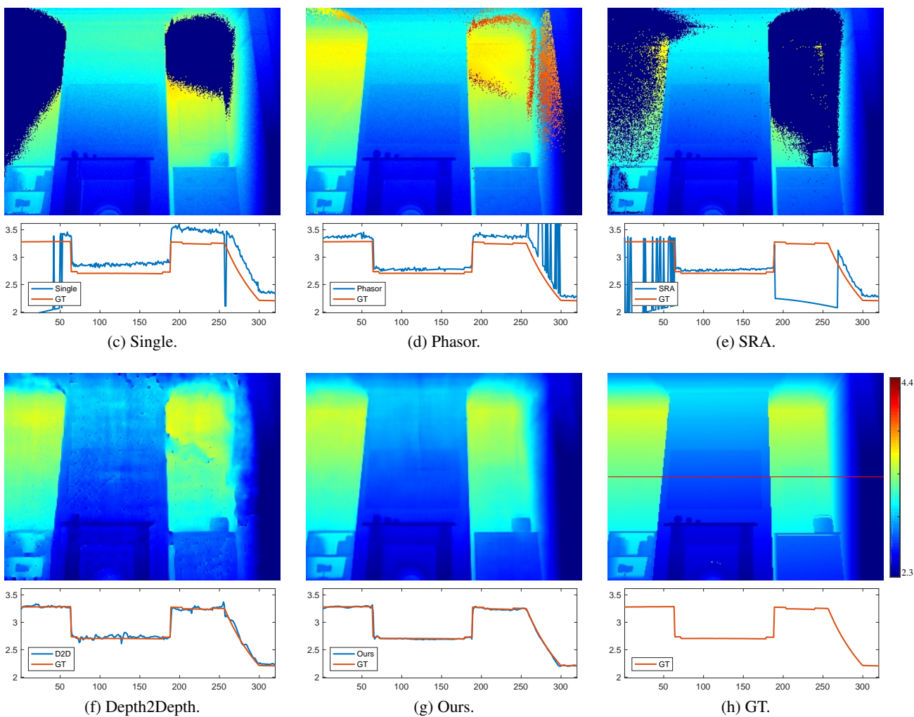
Figure 5: Synthetic results on a common indoor scene with moderate MPI and sensor noise.
