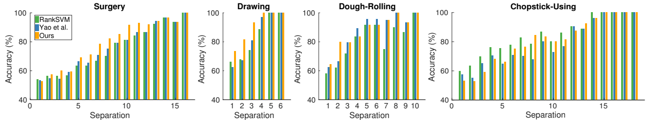
Figure 6. The accuracy of each ordered pair by separation between videos in a pair for each task, in the baselines and our method. The accuracy consistently increases as tested pairs are further in the ground-truth ranking for all datasets.
