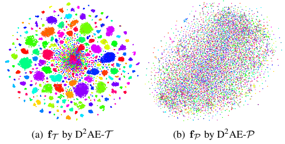
Figure 4. Barnes-Hut t -SNE [30] visualization of the features extracted by two branches (a) D 2 AE- \mathcal{T} and (b) D 2 AE- \mathcal{P} on LFW. The colors indicate different identities. Best viewed in color.
