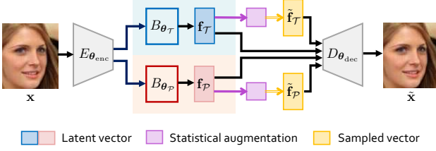
Figure 2. The Distilling and Dispelling Autoencoder model.
