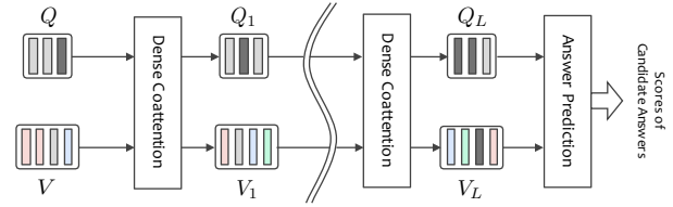
Figure 1: The global structure of the dense co-attention network (DCN).
