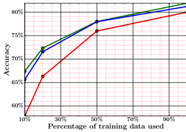
(c) CIFAR 100
