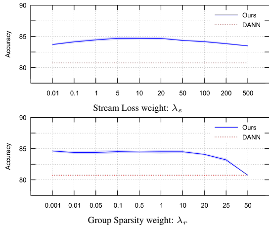
Figure 4: Accuracy as a function of the values of hyperparameters \lambda_s and \lambda_r on the SVHN to MNIST benchmark. It is shown in blue and changes little over a wide range. In practice we take \lambda_s = \lambda_r = 1 . We also plot in red the performance of DANN [8] for comparison purposes.
