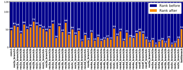
Figure 7: Transformation ranks reduction on the Office dataset for the A \rightarrow W domain adaptation task. The ranks significantly shrink for all layers of the RESNET-50 model.
