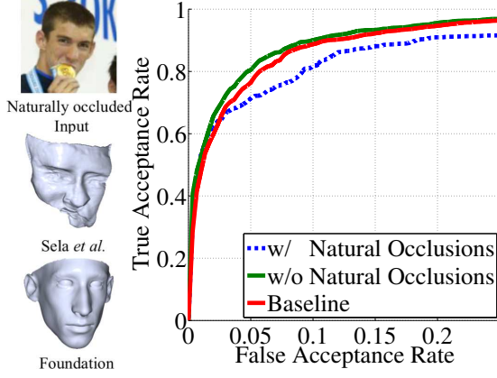
Figure 6: Reconstructions with occlusions. Left: Qualitative results of Sela et al. [43] and the method used as our foundation [51]. The loose regularization required by [43] to produce fine details results in a corrupt shape for the occluded face. The foundation sacrifices details but remains robust. Right: LFW verification ROC for foundation shapes [51], with and without occlusions.
