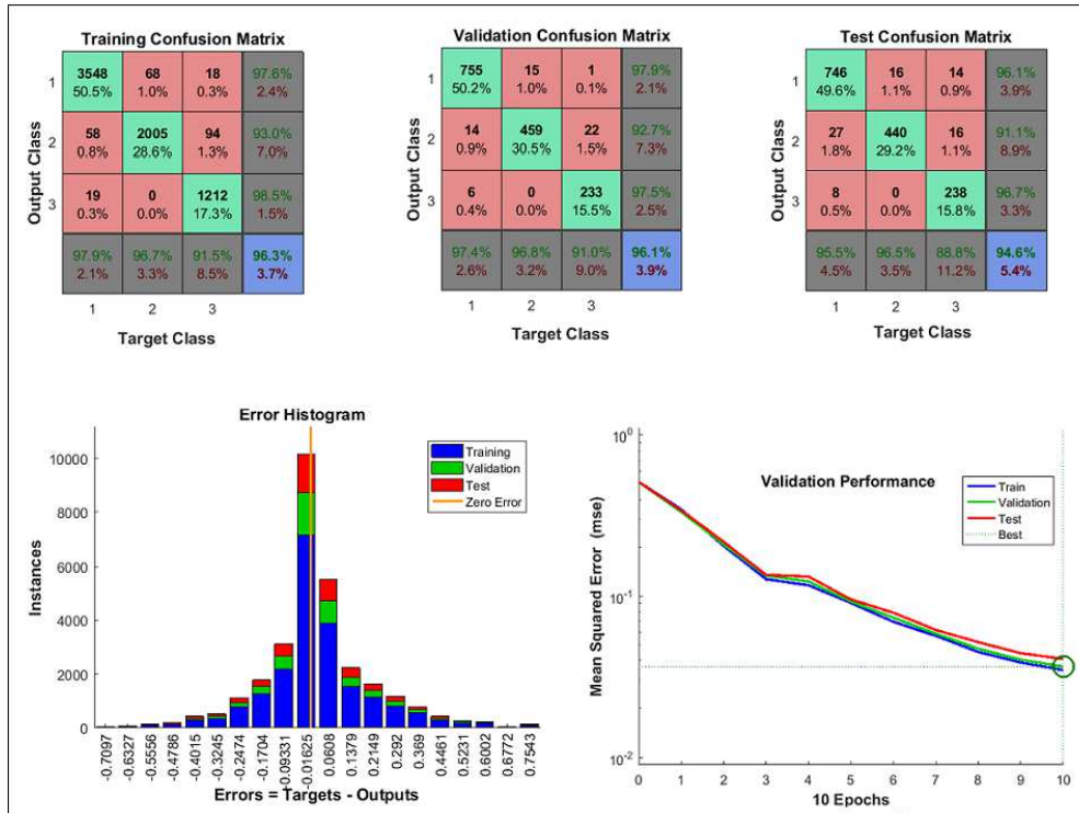
Figure 8. NIST SD27 - Confusion matrix for training, validation and testing, error histogram, and validation performance for the quality assessment neural network. Class 1 = Good, Class 2 = Bad, and Class 3 = Ugly. 7,000 patches were used for training, 1,500 patches for validation and 1,500 patches for testing. The training, validation and testing samples were independently drawn from the dataset. Output Class is the predicted class while target class is the ground-truth class. The fourth row contains Recall values while the fourth column contain the Precision. In the testing confusion matrix, Precision=96.1% and Recall=95.5% for Class 1 means that out of the times Class 1 was predicted, the classifier was correct 96.1% of the time, and out of all the times Class 1 should have been predicted 95.5% of the predictions were correct. The small numbers on all cells but the diagonal (that contains the true positives for the respective classes), as well as the error histogram, and validation performance plots, indicate good classifier performance.
