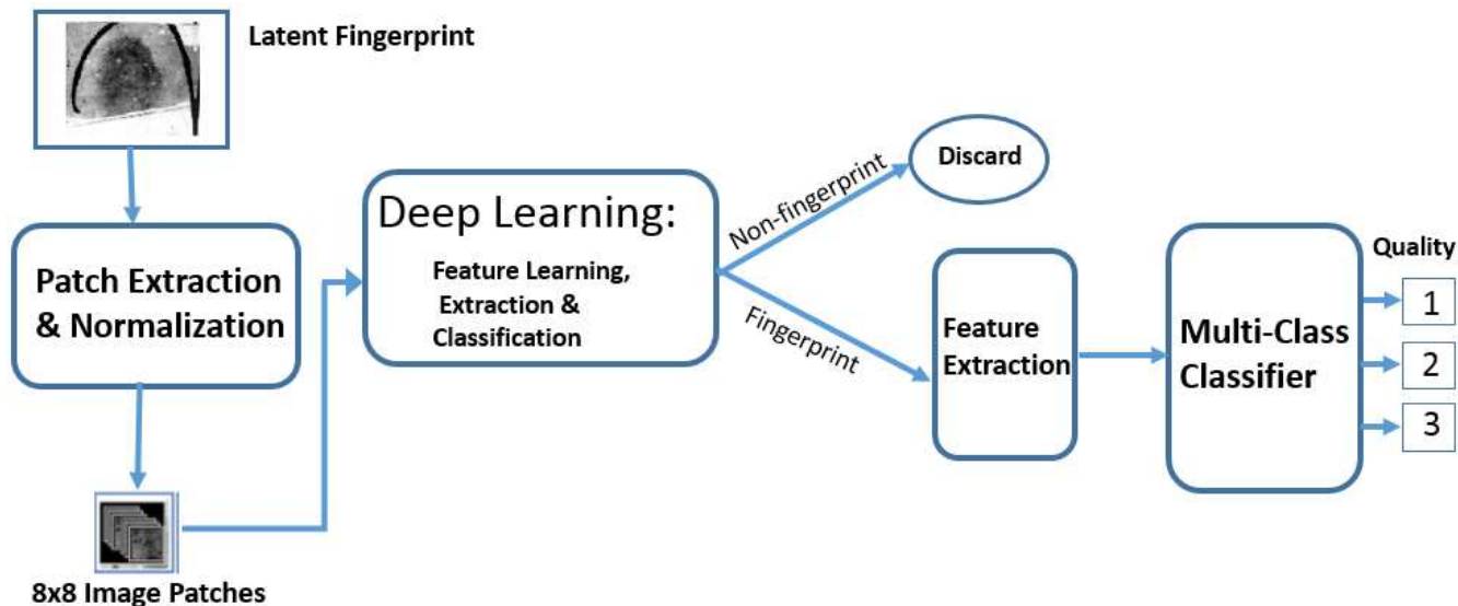
Figure 2. Proposed framework for latent fingerprint quality assessment. The first stage uses a deep learning architecture similar to that in [9], for feature learning, extraction and classification. In the second stage, features are extracted from the segmented fingerprint (ROI) and fed to a multi-class perceptron classifier. The target values from the classifier are 1 (Good), 2 (Bad) and 3 (Ugly).
