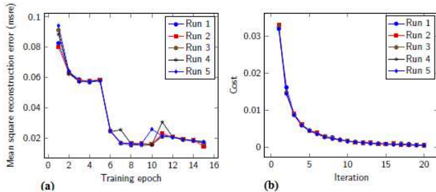
Figure 6. Segmentation Network Stability: (a) shows that the mean square reconstruction error (MSRE) during the pre-training phase for the 5 runs followed similar trajectories. Similarly, (b) shows that the error during the fine-tuning phase for the 5 runs were close. These results are indicative of the stability of the network.
