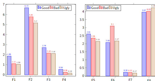
Figure 4. Gabor features used to train the multi-class perceptron classifier for image patch quality assessment. The features were computed from the kurtosis and skewness of the Gabor filter responses of the image patches. F1 and F4 are the peak and mean skewness of the magnitude response, respectively. F2 and F5 are the peak and mean kurtosis of the phase response, respectively. F3 is the mean kurtosis of the magnitude response. F6 and F7 are the peak and mean skewness of phase response, and F8 is the peak of the magnitude response. F7 was scaled up by 0.2 for visibility. The charts show that together, the features exhibit discriminative potential for classifying patches into good, bad and ugly bins.
