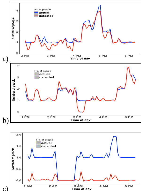
a) b) c) Figure 2. LOESS curve for actual and detected number of visitors for three different patients a) patient 1, sufficient lighting (daytime), b) patient 2, sufficient lighting (daytime), and c) patient 3, insufficient lighting (nighttime).
