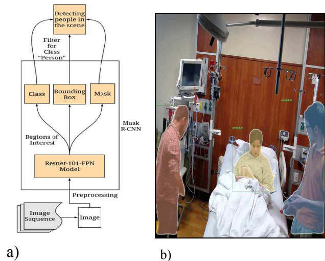
a) b) Figure 1: a) The end-to-end pipeline for detecting the visitations in the ICU. b) Image from a simulated ICU video with mask over the persons detected by Mask R-CNN
