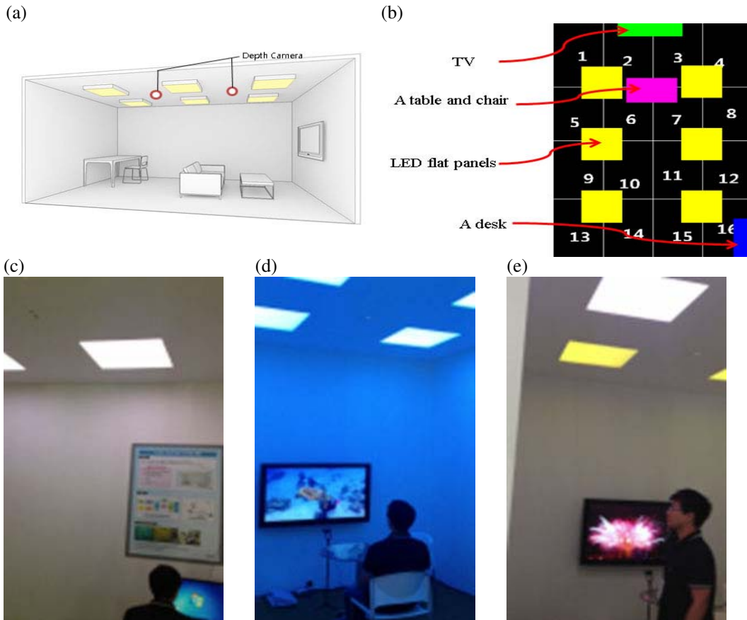
Figure 7. Schematic diagram of the smart lighting living room, and the lighting panels and furniture locations on the global map and captured sample scenes in different activity modes:(a) A schematic diagram of the smart lighting living room, (b) Global and lighting source location, and furniture location, (c) Sample scenes of lighting control in different modes; left:study mode, middle: watching TV mode, right: walking around mode.
