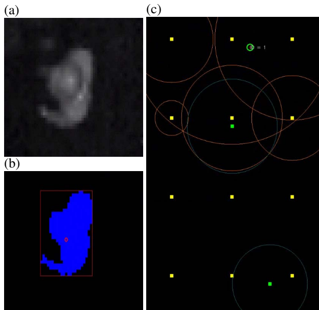
Figure 4. Human detection and control of lighting from thermal camera: (a) Original thermal image, (b) Depth human and its center, (c) Lighting control based estimated person location from thermal camera.
