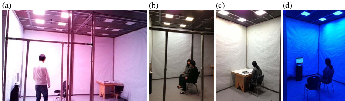
Figure 9. Evaluation of the energy saving based on the activity mode evaluation:(a) walking around mode, (b) dialogue mode, (c) study mode, (d) watching TV mode.
