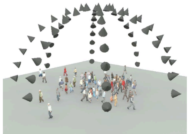
Figure 2. Simulated crossing scene along with the 64 camera configurations used to obtain the dataset.
