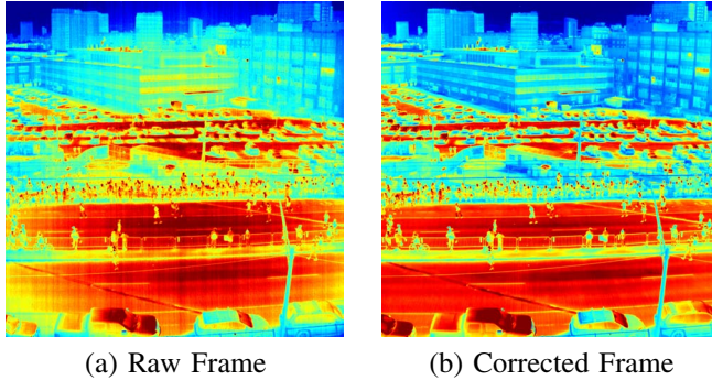
Figure 2. Sample images for nonuniform correction.
