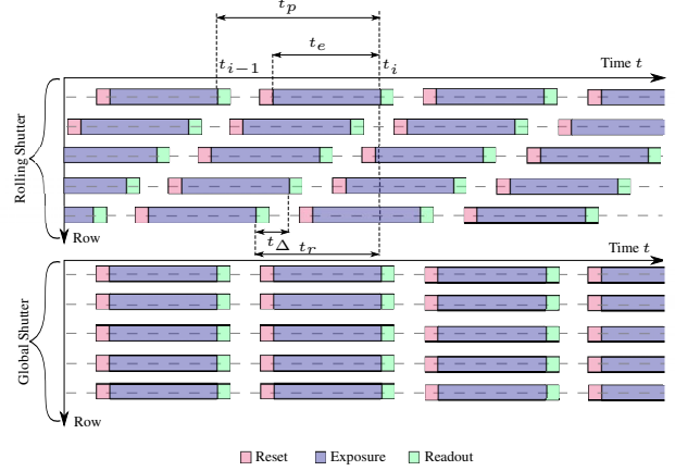
Figure 1. Top, RS camera model. Each raw of the sensor is sequentially exposed during a fixed exposure time t_e . The total readout time t_r is the delay between the readout of the first and the last row. The frame period t_p is the time delay between the readout of the same raw of the image. Bottom, global shutter mode. All rows of the image are exposed simultaneously during a fixed exposure time t_e .
