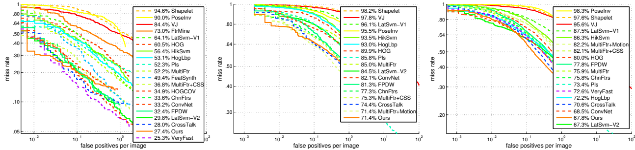
Figure 4: From left to right: performance on INRIA, TUD-Brussels and ETH test set. Algorithms are sorted using the partial AUC score in the FPPI range [0, 0.1] . Our pAUCs consistently performs comparable to the state-of-the-art.
