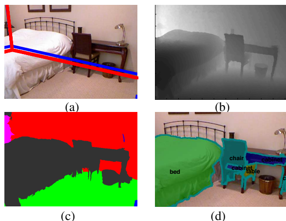
Figure 1. Inferring layout, clutter and semantic classes: The input image with layout prediction result (blue) and ground truth (red) overlaid is shown in (a), the depth map employed is shown in (b). (c) and (d) show our inferred labeling and segmentation.
