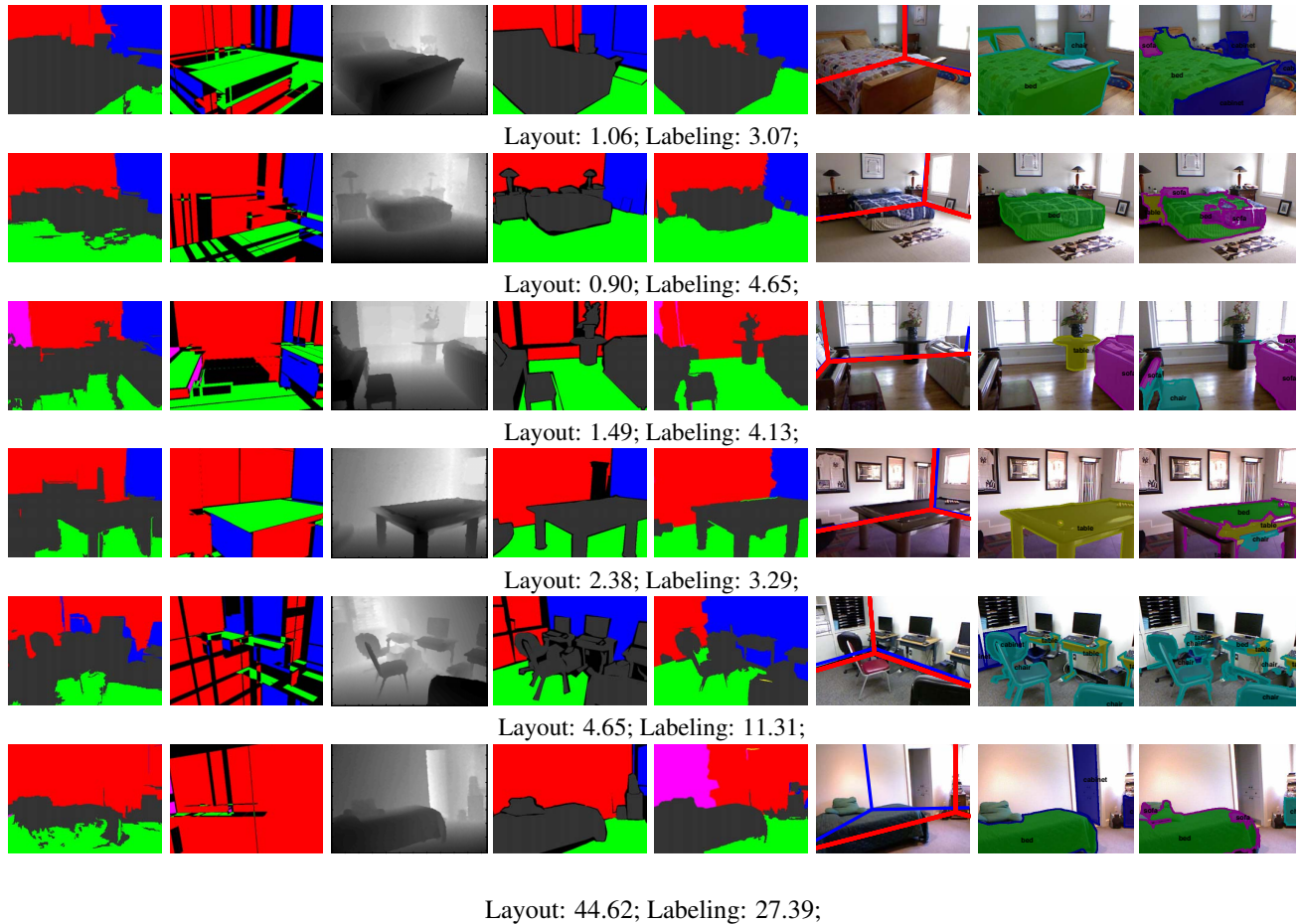
Figure 5. Qualitative results: In the first three columns we show OM, GC and depth. In the fourth and fifth column we show the ground truth labeling as well as our labeling estimation. The sixth column depicted the layout estimates in (blue) and the ground truth in red. Finally the last two columns depicted the semantic labeling for the ground truth as well as our estimates. A failure mode due to bad vanishing points is illustrated in the last row.
