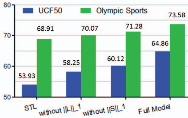
Figure 7. Classification accuracy of different methods (STL, our model without \|L\|_1 , our model without \|S\|_1 and our full model) on the UCF50 data set using 25% of the training data and on the Olympic Sports data set.
