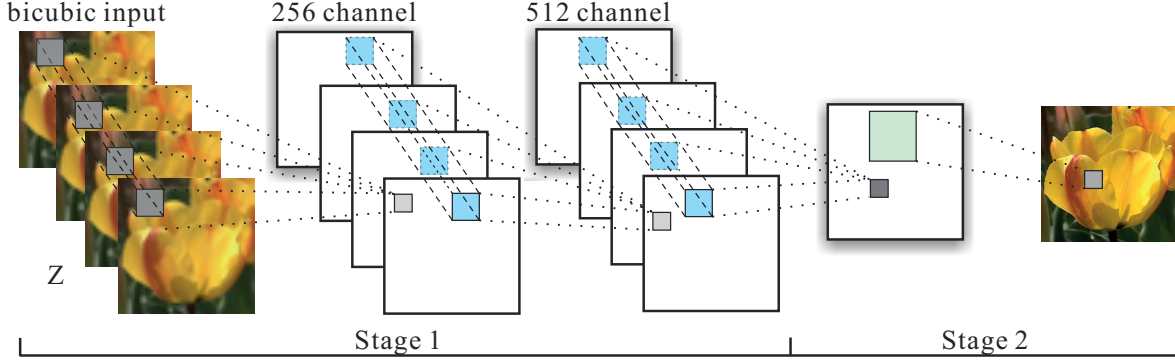
Figure 3. The two-stage architecture of our CNN framework. The input is a multi-channel image containing the set of reconstructed blurred HR images and the bicubic interpolated reference frame. The first and second stages aim at merging SR drafts and final deconvolution respectively.
