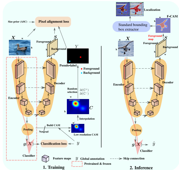
Figure 2: Our proposal: training (left), inference (right).
