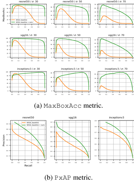
Figure 5: Localization accuracy as a function of threshold value \tau for CAM* (orange) and CAM* + ours (green). (A) CUB. (b) OpenImages.
