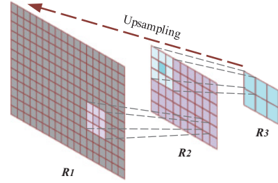
Figure 5. ROI feature fusion architecture.
