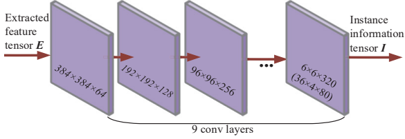
Figure 4. Instance attention module (IAM) architecture.
