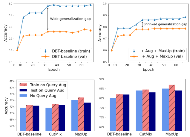
Figure 6: Accuracy results for training and validation on R2-D2 base-learner [7] with a DBT-regularized ResNet-12 backbone on the CIFAR-FS dataset. (Top Left) Baseline model and (Top right) Augmentation "Aug" and MaxUp. The MaxUp augmentation strategy narrows down the generalization gap and reduces overfitting. (Bottom left) 1-shot classification and (Bottom Right) 5-shot classification for Query data augmentation.
