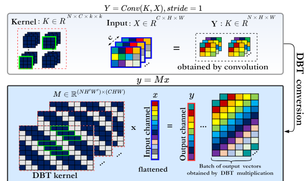
Figure 1: The convolution expression; \text{Conv}(K, X) is converted into a faster DBT vector representation; y = Mx .
