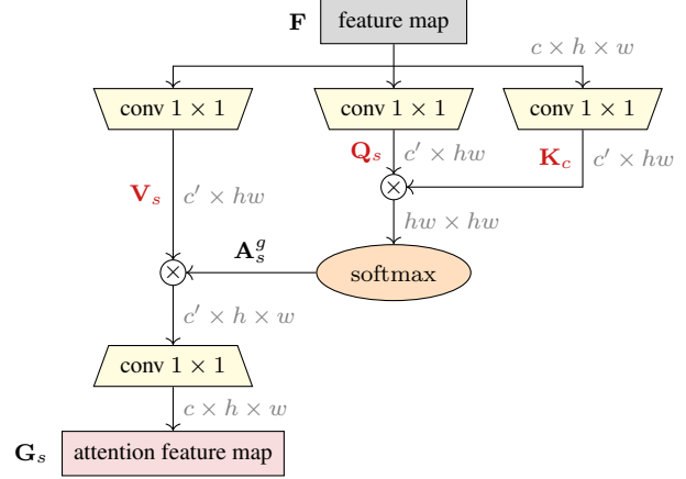
Figure 5. Global spatial attention.
