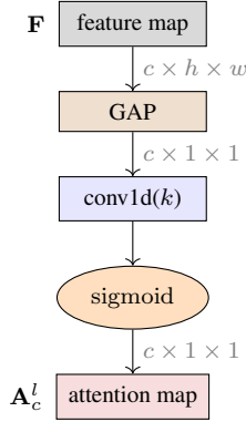
Figure 2. Local channel attention.
