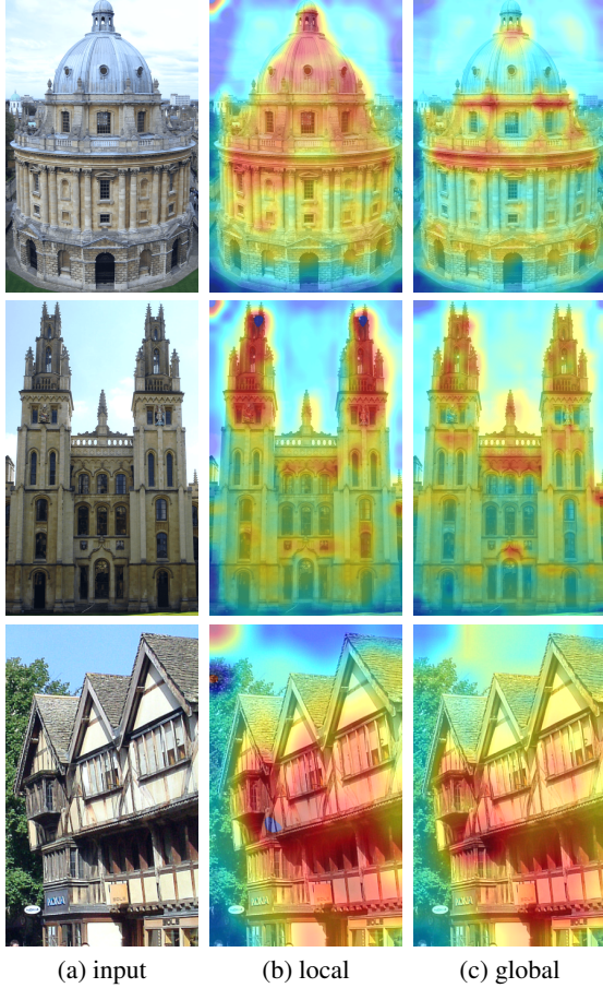
Figure 6. Local and global spatial attention. Left: input images. Middle: local spatial attention heat maps. Right: global spatial attention heat maps. Red (blue) means higher (lower) attention weight.
