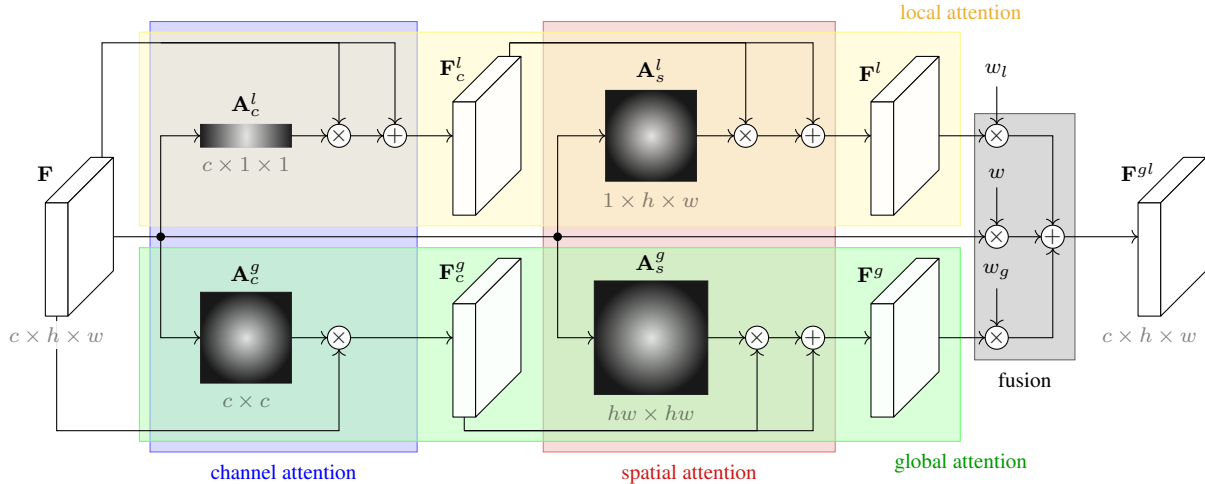
Figure 1. Our global-local attention module (GLAM) involves both channel and spatial attention, as well as both local attention (channels/locations weighted independently, based on contextual information obtained by pooling) and global attention (based on pairwise interaction between channels/locations). As a result, four attention maps are used: local channel ( \mathbf{A}_c^l ), local spatial ( \mathbf{A}_s^l ), global channel ( \mathbf{A}_c^g ) and global spatial ( \mathbf{A}_s^g ). The input feature map \mathbf{F} is weighted into local ( \mathbf{F}^l ) and global ( \mathbf{F}^g ) attention feature maps, which are fused with \mathbf{F} to yield the global-local attention feature map \mathbf{F}^{gl} . The diagram is abstract: The four attention modules are shown in more detail in Figures 2, 3, 4, 5.
