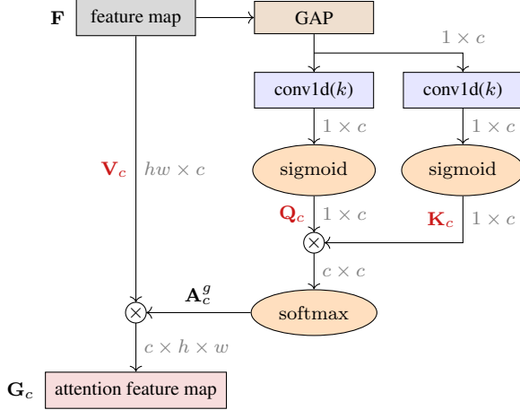
Figure 4. Global channel attention.
