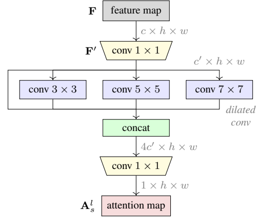
Figure 3. Local spatial attention. Convolutional layers in blue implemented by dilated convolutions with kernel size 3 \times 3 and dilation factors 1, 3, 5.
